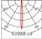
XP-E2 10° 3000K
